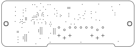
Drill Map:
